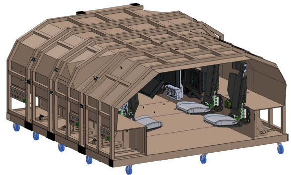
Inside View of Modular Mobile Crewstation Simulator
