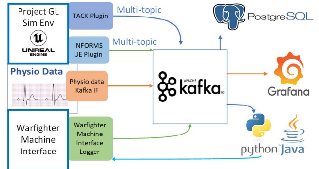
Apache Kafka based architecture for data stream management and synchronization, storage options for search and exploration
